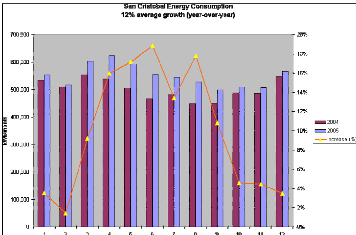
Figure 4: San Cristobal monthly energy consumption 2004-2005 3
