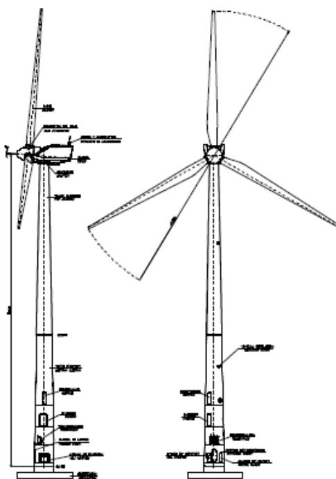
Figure 2 Machine scheme
